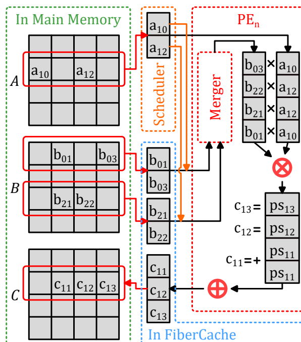
Figure 2.5 – Gamma Dataflow
