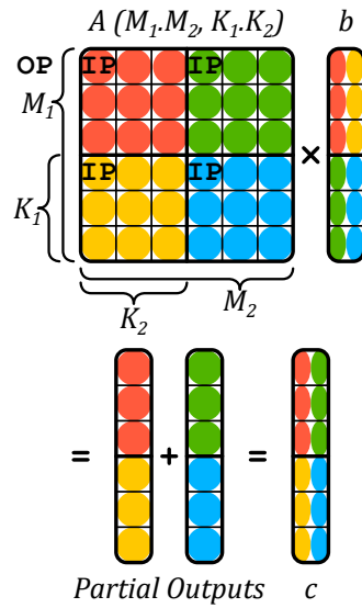
Figure 1.5: An Example of Tiling on SpMV
