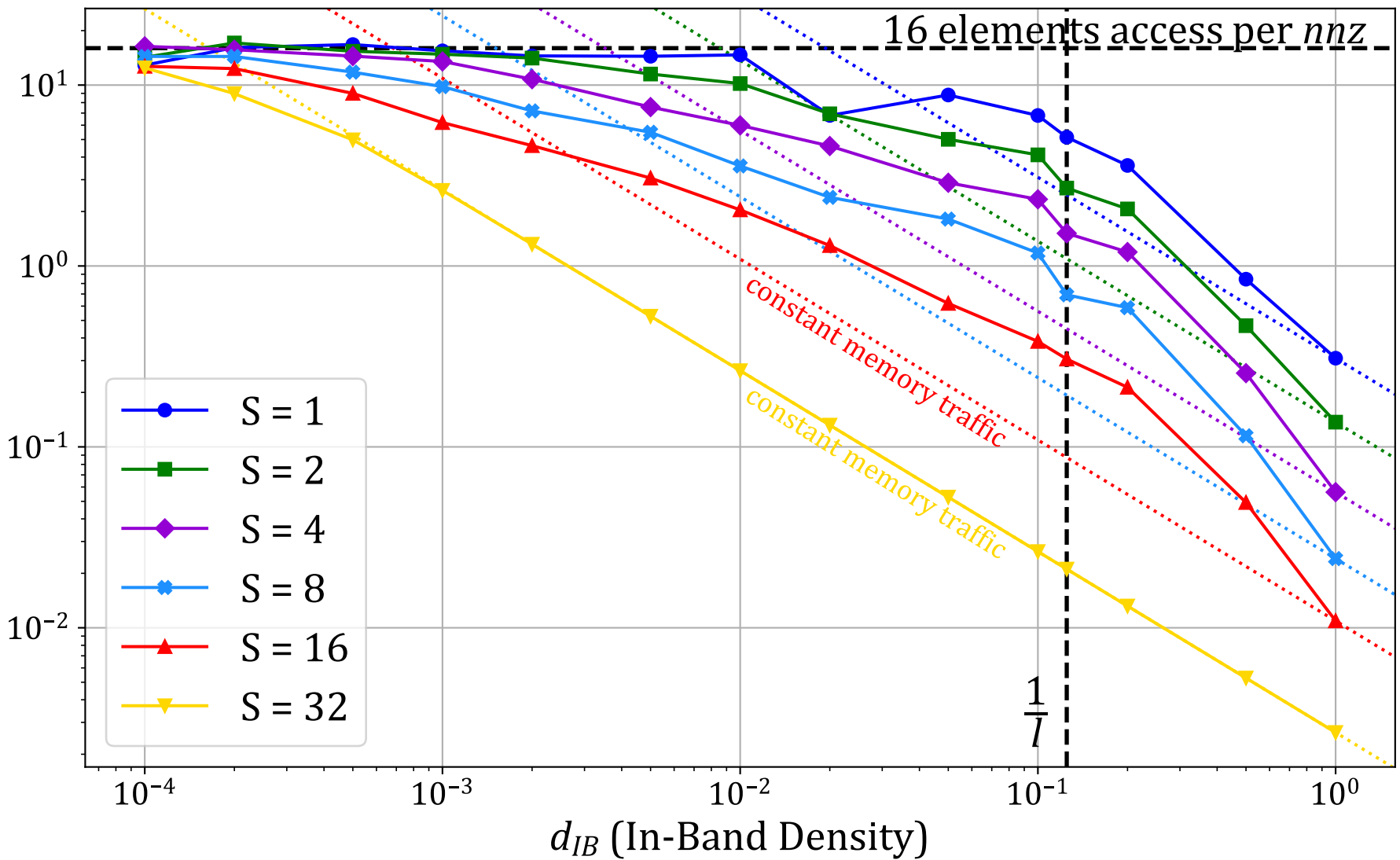
Normalized Memory Traffic
