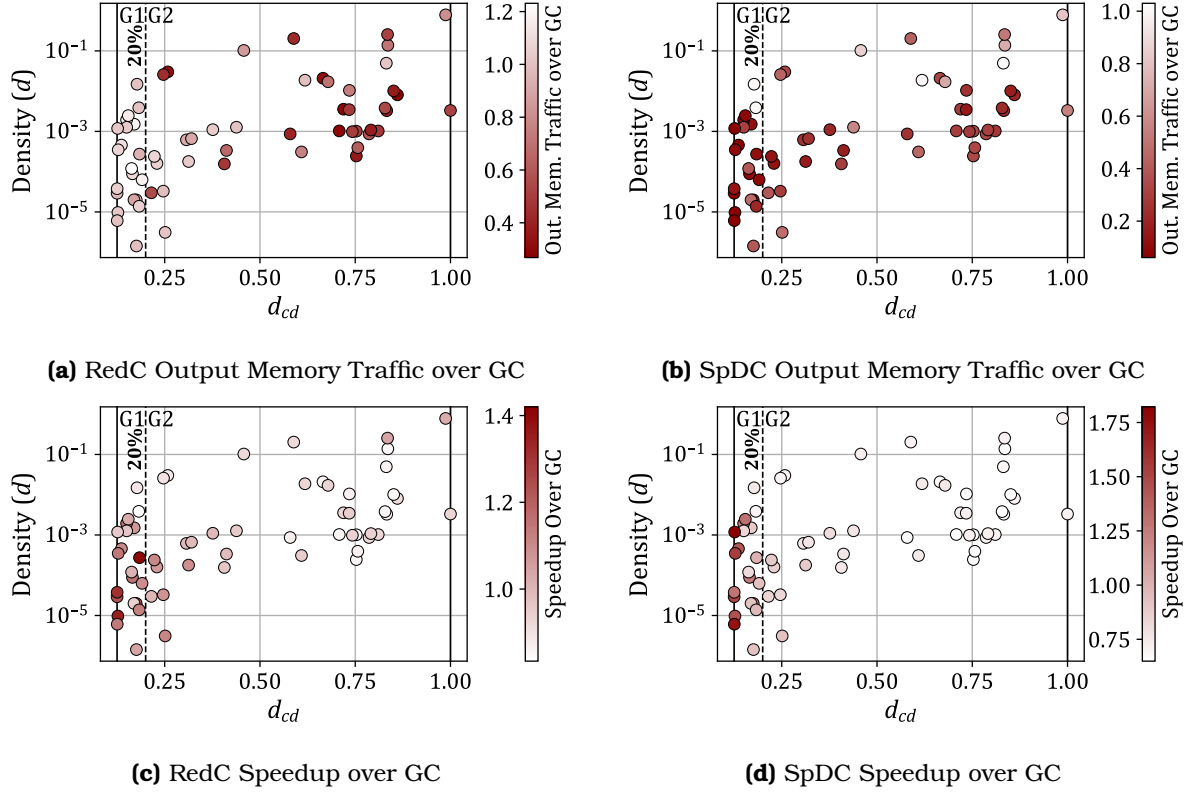
Figure 5.10: Memory Traffic and Speedup Performance Visualized Across Benchmark Matrix Densities and d_{cd}
