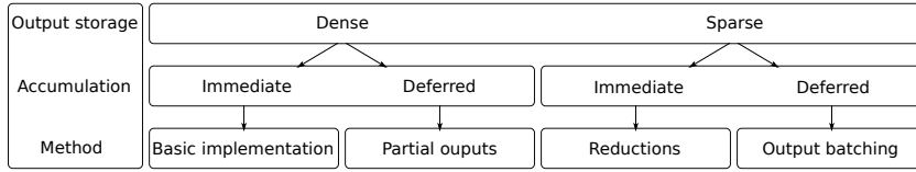
Figure 1.4: Strategies for Dealing with Random Output Updates in Outer Product Algorithms
