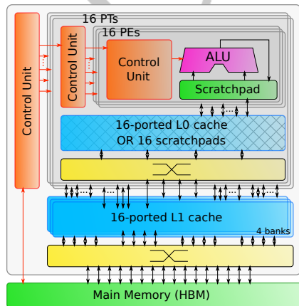
Figure 2.1: Architecture of OuterSPACE
