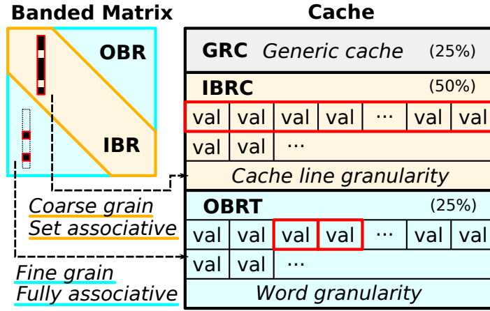
Figure 2.3: Data-Cache Partitioning into Regions (GRC, IBRC, OBRT)
