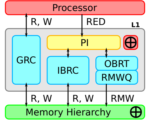
Figure 2.4: Simplified View of the Memory Hierarchy with SpDCache
