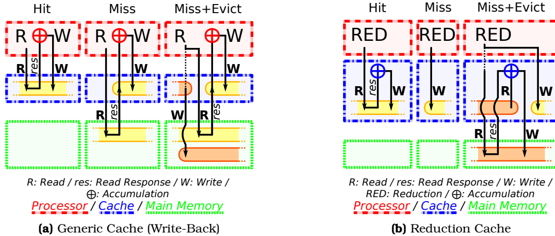
Figure 2.1: Read (R) and Write (W) Transactions of a Reduction Operation in Generic and Reduction Caches (TODO there is place: put legend on the side)
