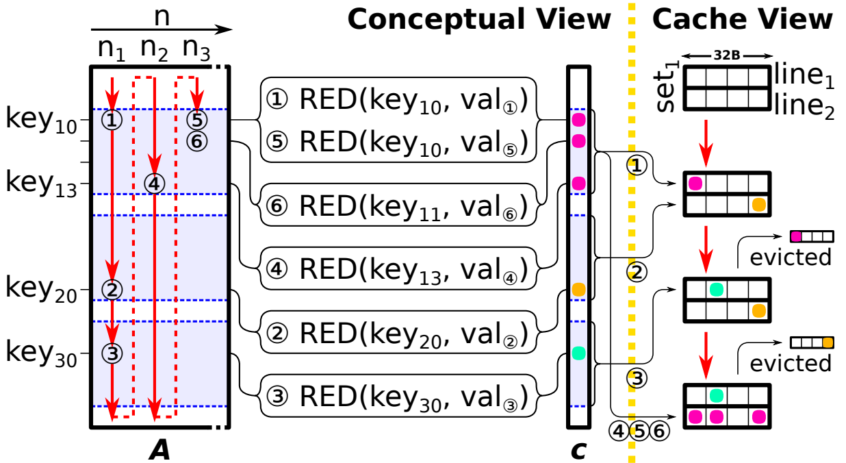
Figure 2.2: Traversal of Non-Zero Elements of Input Matrix for OP SpMV (left) and Impact on Cache (right)
