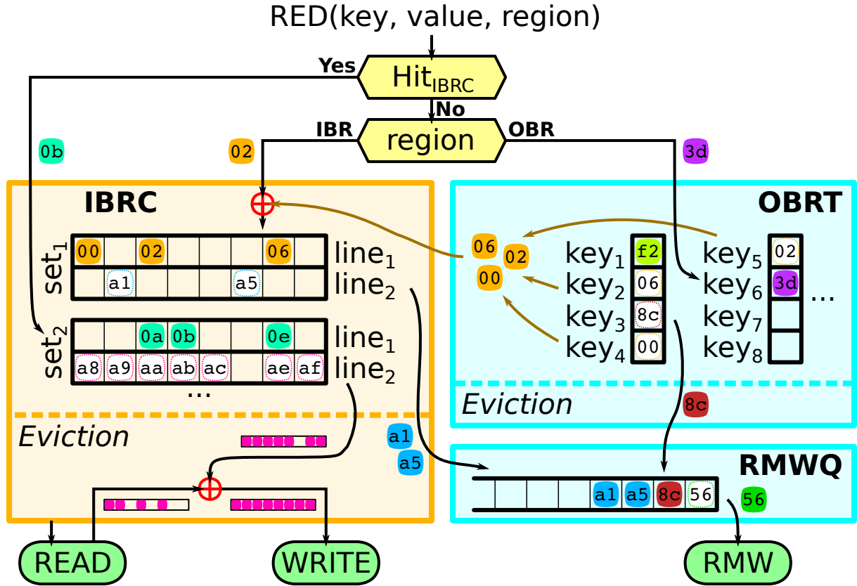
Figure 2.5: Internal Operation of SpDCCache with Examples
