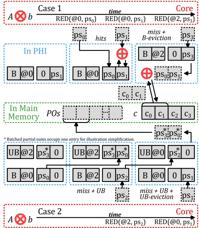
Figure 2.7 – PHI Dataflow
