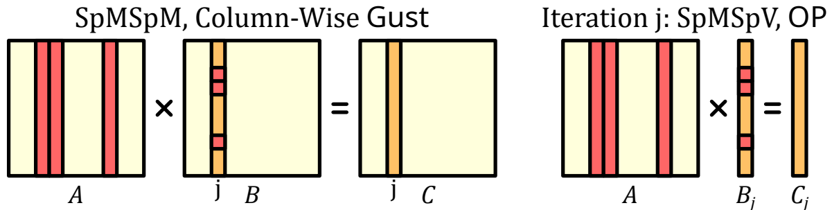
Figure 6.1 – Gustavson SpMSpM Kernel with an Outer-Product SpMSpV Iteration
