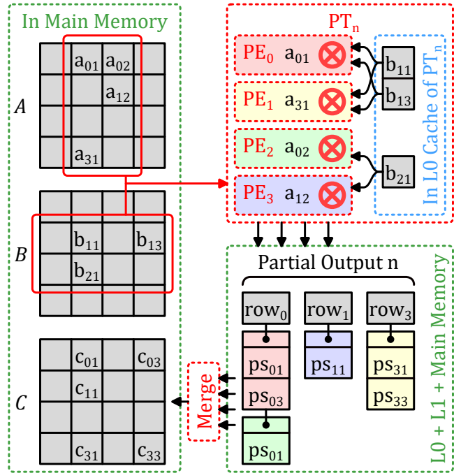
Figure 2.2 – OuterSPACE Dataflow
