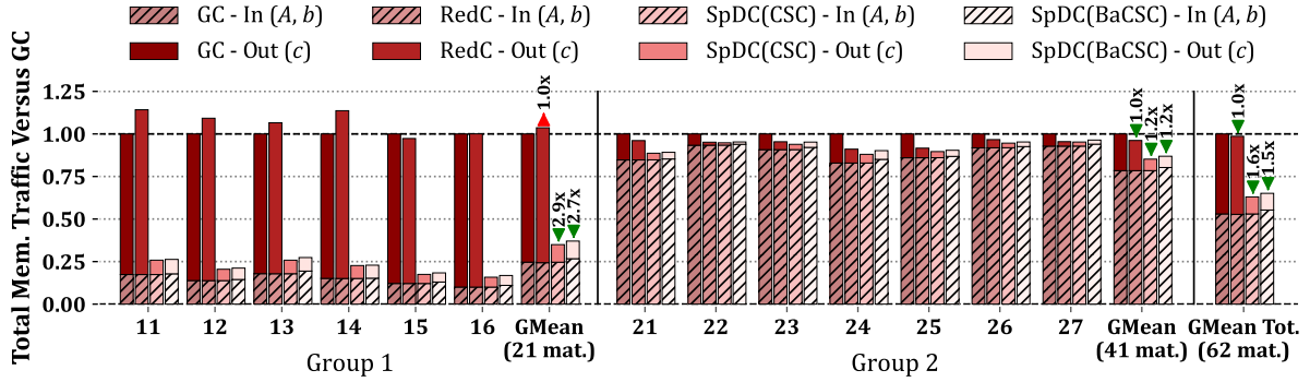
Figure 5.8 – Total Memory Traffic for Input Matrix A , Input Vector b and Output Vector c , Normalized Compared to GC, Measured from RTL Simulations
