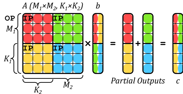
Figure 1.4 – An Example of Tiling on SpMV
