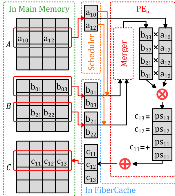
Figure 2.5 – Gamma Dataflow
