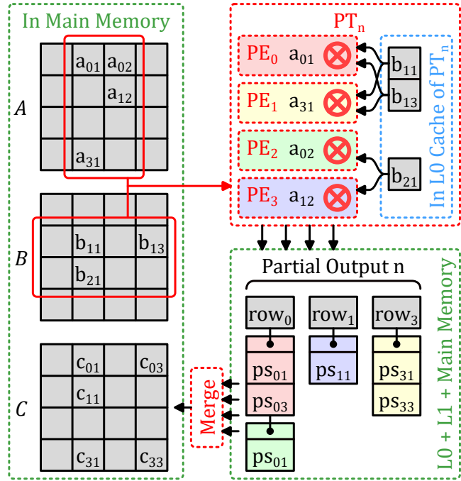
Figure 2.2 – OuterSPACE Dataflow
