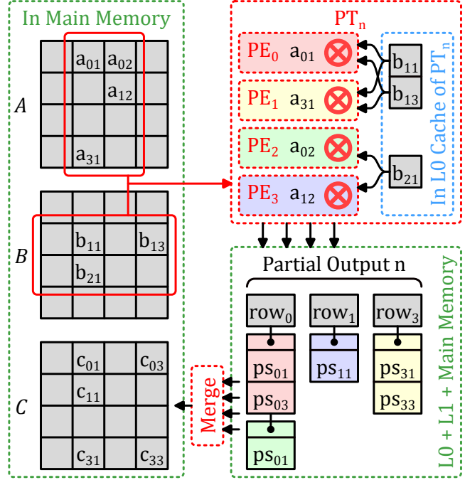
Figure 2.2 – OuterSPACE Dataflow
