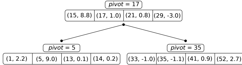
Figure 2.10: VBST Data Structure Used by SortCache
