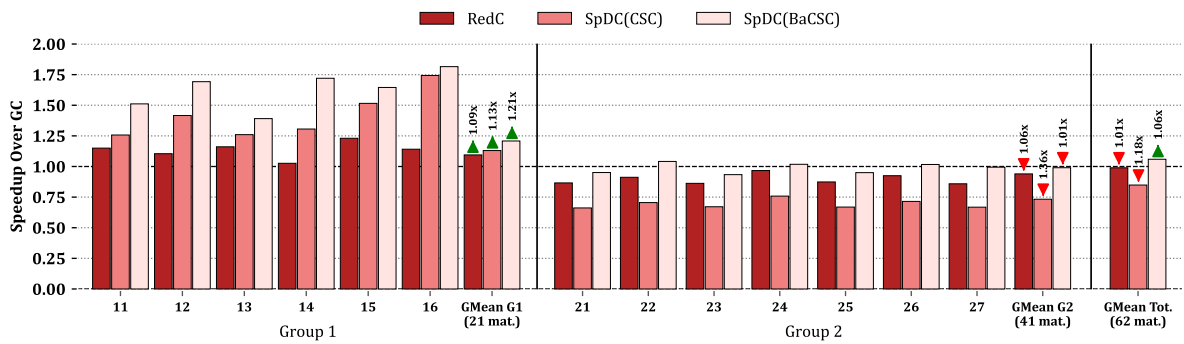
Figure 5.9: Normalized Speedup
