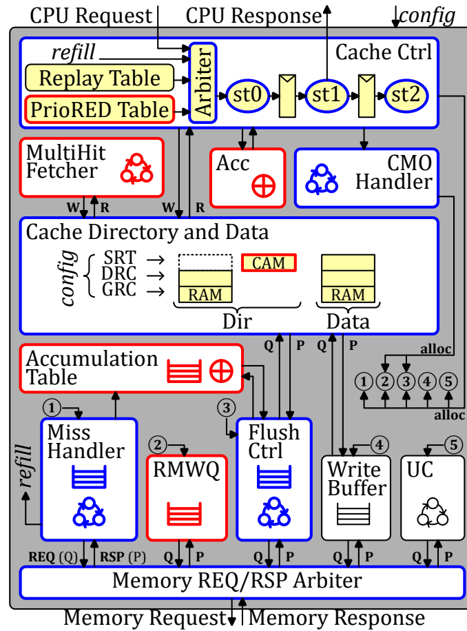
Figure 5.1 – SpDCache Microarchitecture, based on HPDcache
