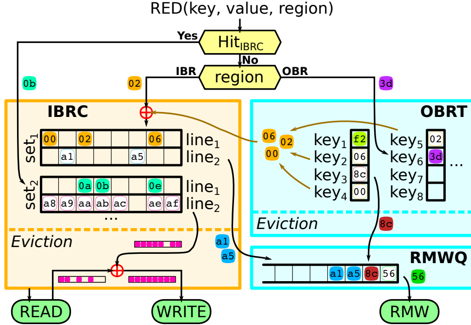
Figure 2.5: Internal Operation of SpDCache with Examples TODO: update region names
