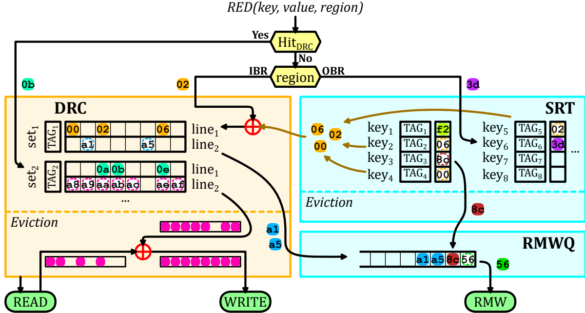
Figure 3.5: Internal Operation of SpDCache with Examples
