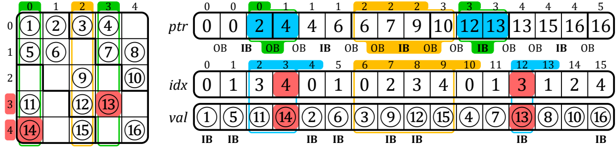
Figure 1.2: Example of a Sparse Matrix in BaCSC Format
