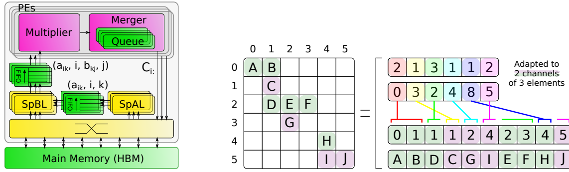
Figure 2.6: Architecture of Figure 2.7: (FL, UOP, CP) Channel-Major Format MatRaptor (C^2SR)
