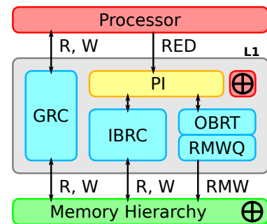
Figure 3.4: Simplified View of the Memory Hierarchy with SpDCache
