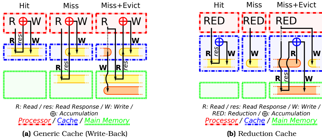
Figure 3.1: Read (R) and Write (W) Transactions of a Reduction Operation in Generic and Reduction Caches (TODO there is place: put legend on the side)
