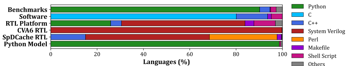
Figure C.2 – Programming Language Distribution Across All Working Repositories
