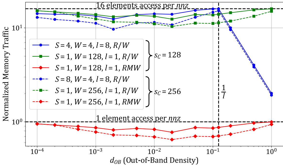
Figure 4.6: Normalized Output Memory Traffic of the Out-of-Band, Depending on the Density for Several Cache-Sizes
