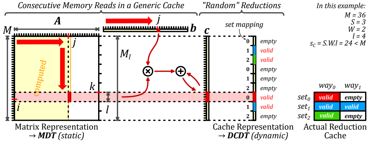
Figure 4.2: Input Matrix and Cache Representation of the Model
