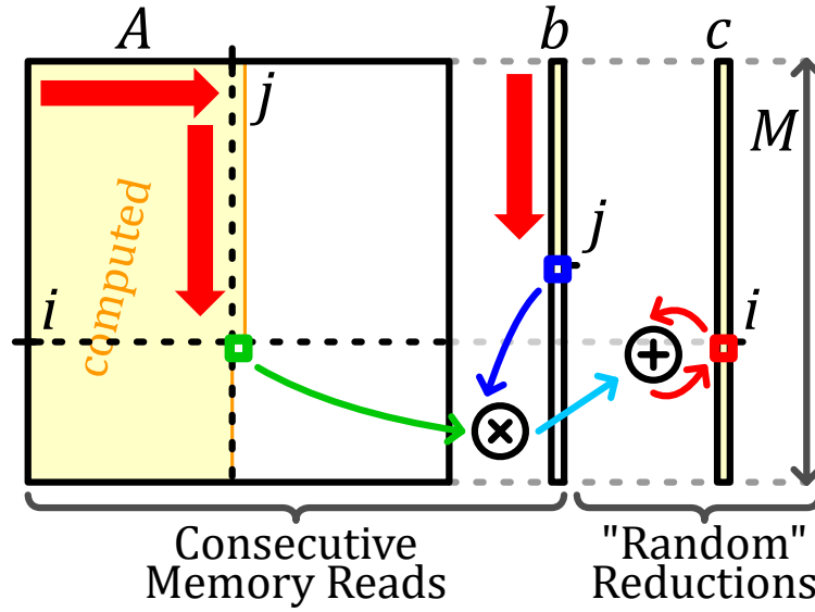
Figure 4.1: Visual Representation of OP SpMV Computation
