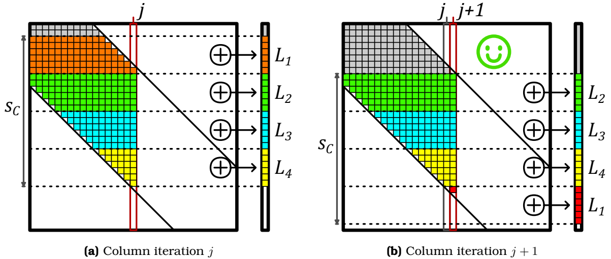
Figure 4.4: Example of the Eviction Rotation in a Perfect Band when the Cache is ‘Properly’ Sized ( s_C = w_B + l - 1 )
