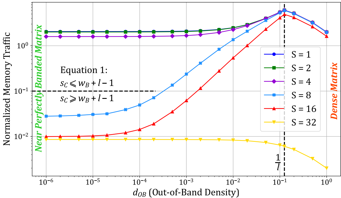
Figure 4.5: Normalized Output Memory Traffic Depending on the Out-of-Band Density for Several Cache-Sizes
