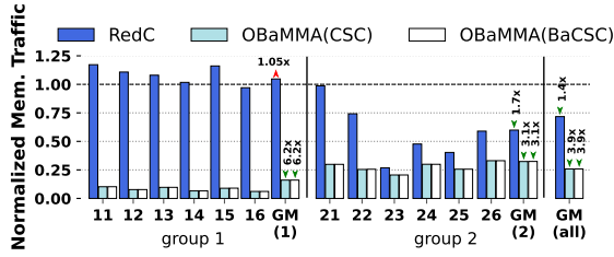
Figure 5.7: Normalized Output Memory Traffic
