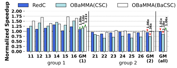
Figure 5.8: Normalized Speedup
