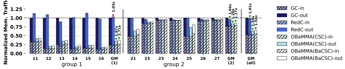
Figure 5.9: Normalized Memory Traffic on Input Matrix, Input Vector and Output Vector
