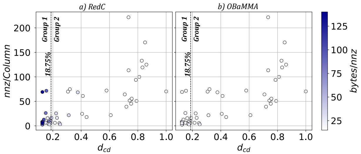
Figure 5.10: Scatter Plot of Normalized Memory Traffic for Benchmark Matrices ( d_{cd} vs nnz/Column ) in bytes/nnz
