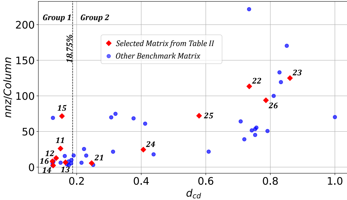
Figure 5.6: Benchmark Matrices: d_{cd} vs nnz/Column
