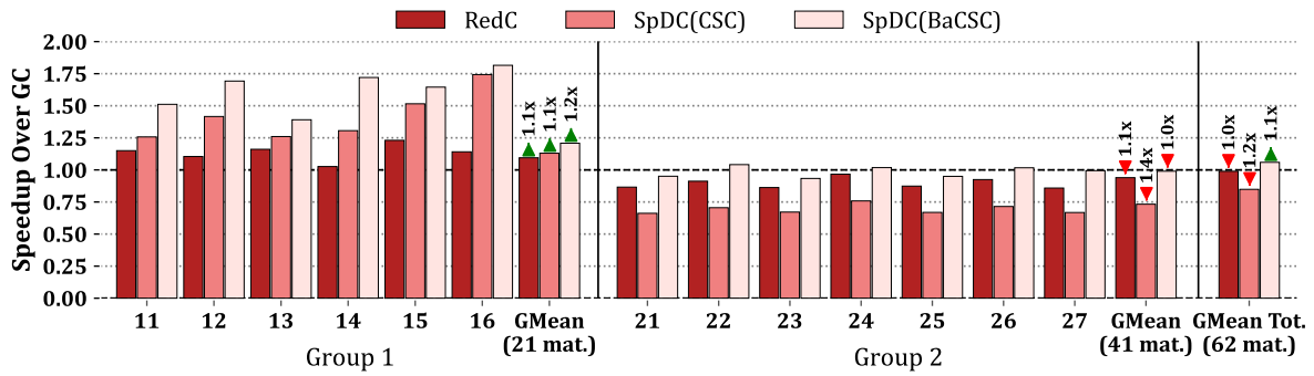
Figure 5.9: Speedup over GC, from RTL Simulations
