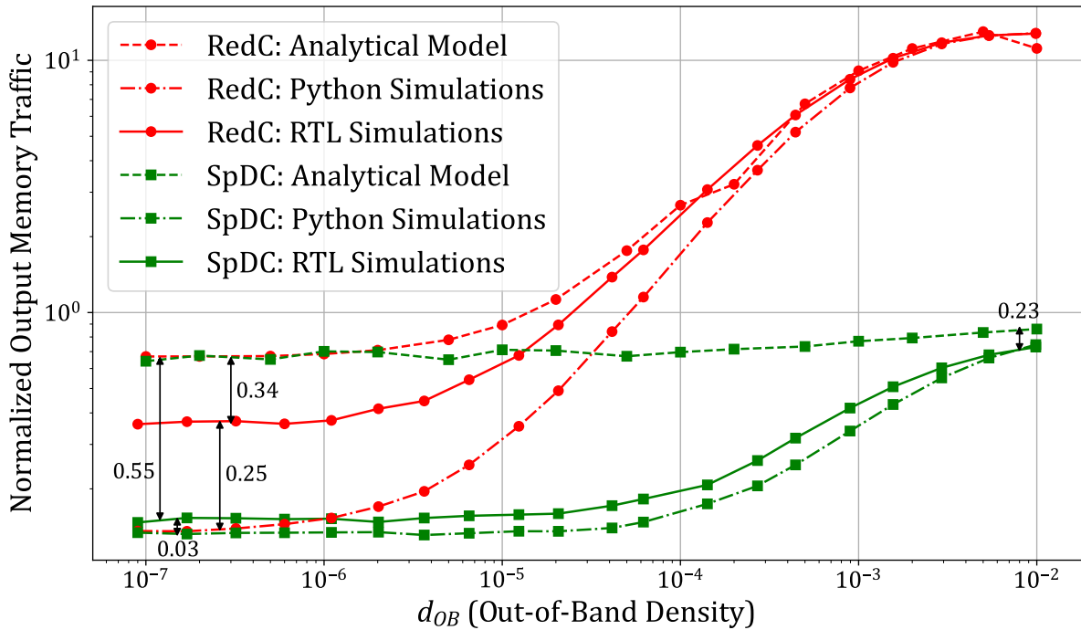
Figure 5.5: Normalized Output Memory Traffic Depending on the Out-of-Band Density for the RedC and SpDC Configurations, Through Different Simulation Models
