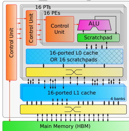
Figure 2.1: Architecture of OuterSPACE
