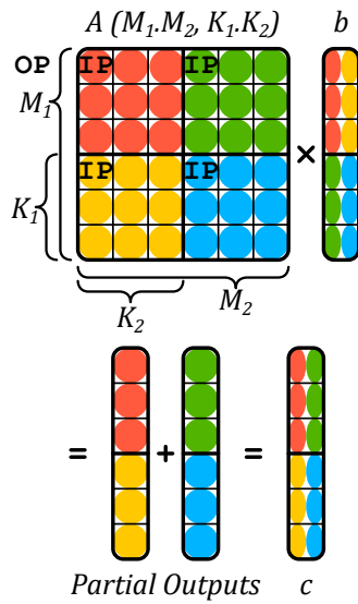
Figure 1.3: An Example of Tiling on SpMV
