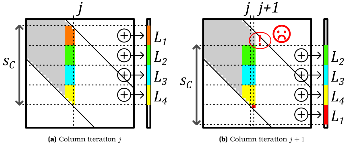
Figure 4.3: Example of the Eviction Rotation in a Perfect Band when the Cache is Undersized ( s_C < w_B + l - 1 ) redo? there is space, clarify where is c
