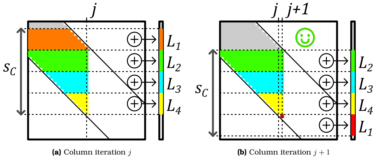
Figure 4.4: Example of the Eviction Rotation in a Perfect Band when the Cache is ‘Properly’ Sized ( s_C = w_B + l - 1 )
