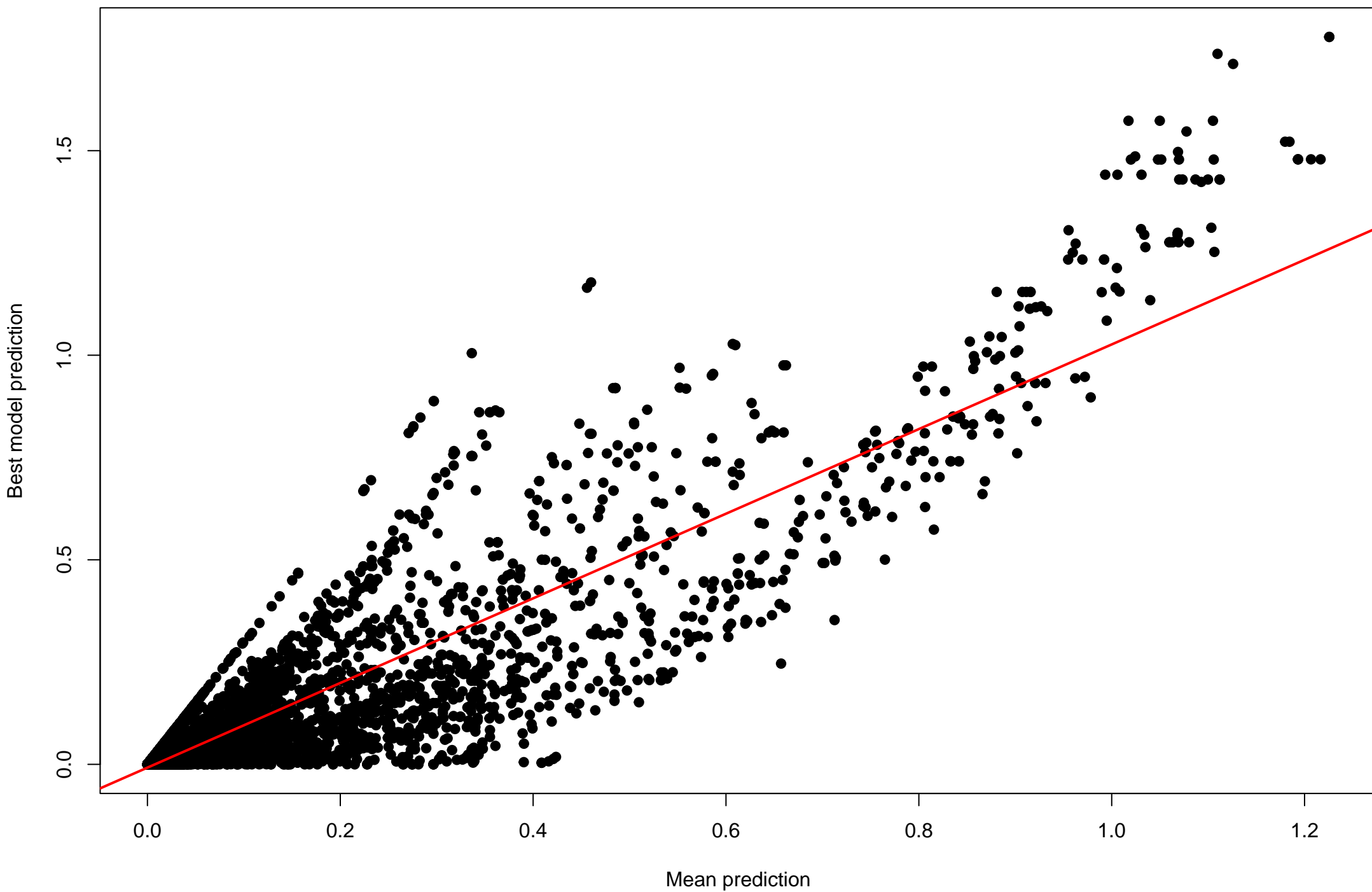
Best model prediction vs Mean prediction ( R^2 = 0.813 )
