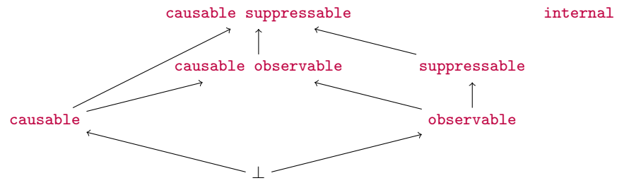
Fig. 1: Capability lattice
