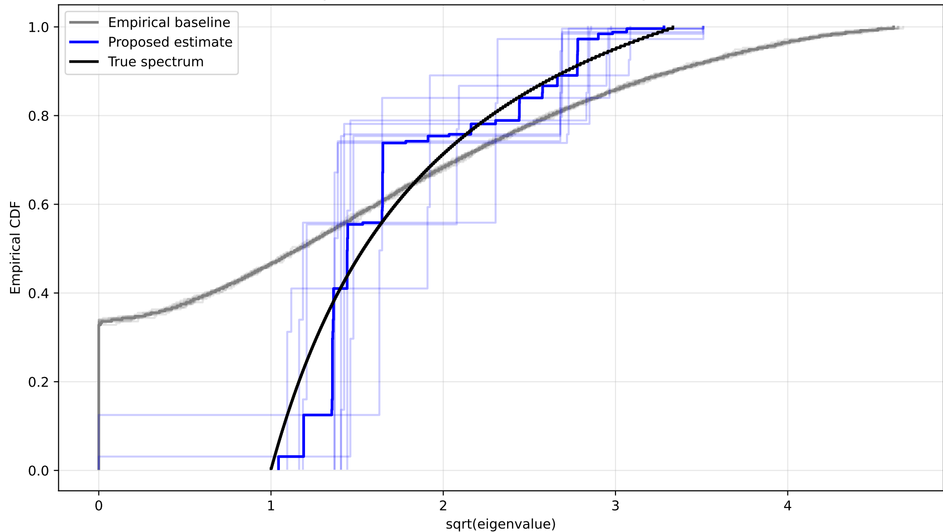
Identity covariance under heteroskedastic diagonal noise
