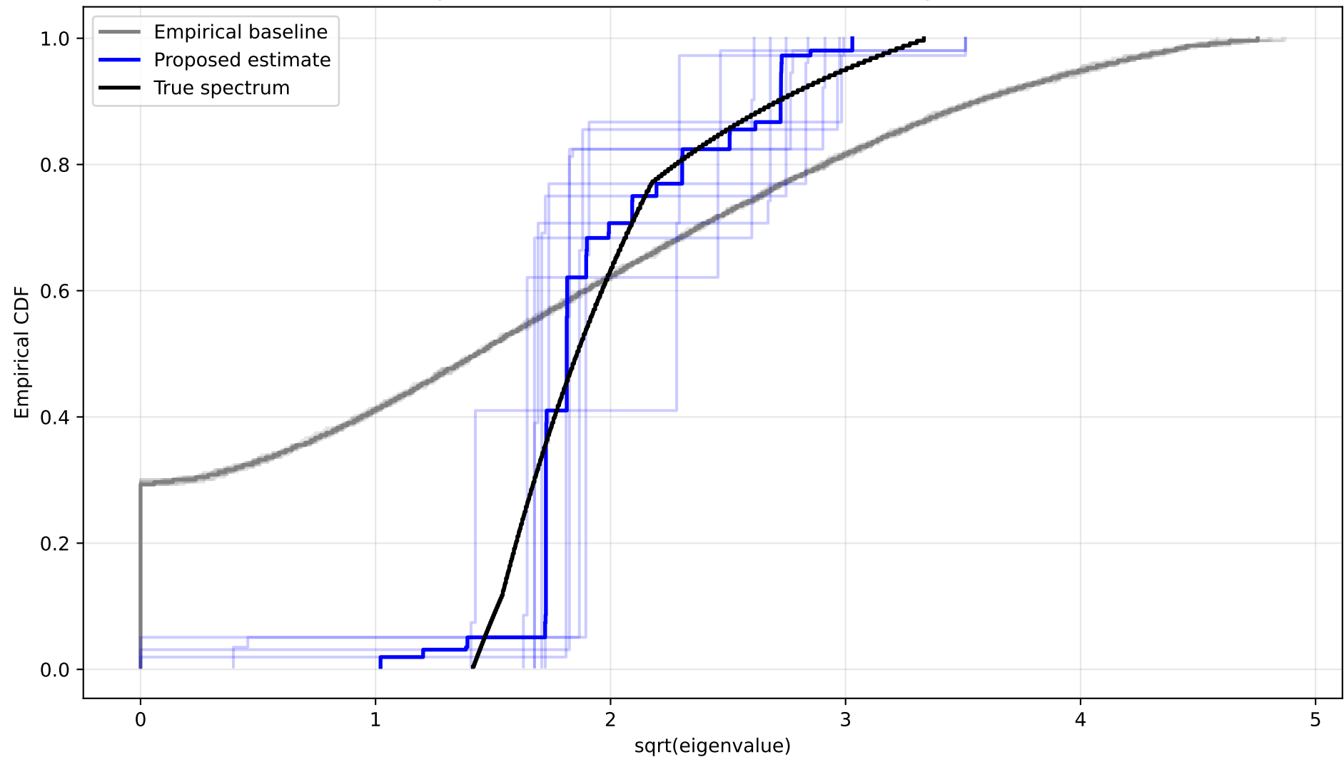
Two-spike covariance under heteroskedastic diagonal noise
