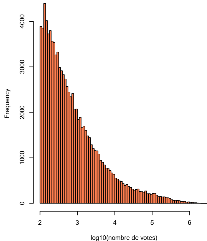
Distribution log10(votes)
