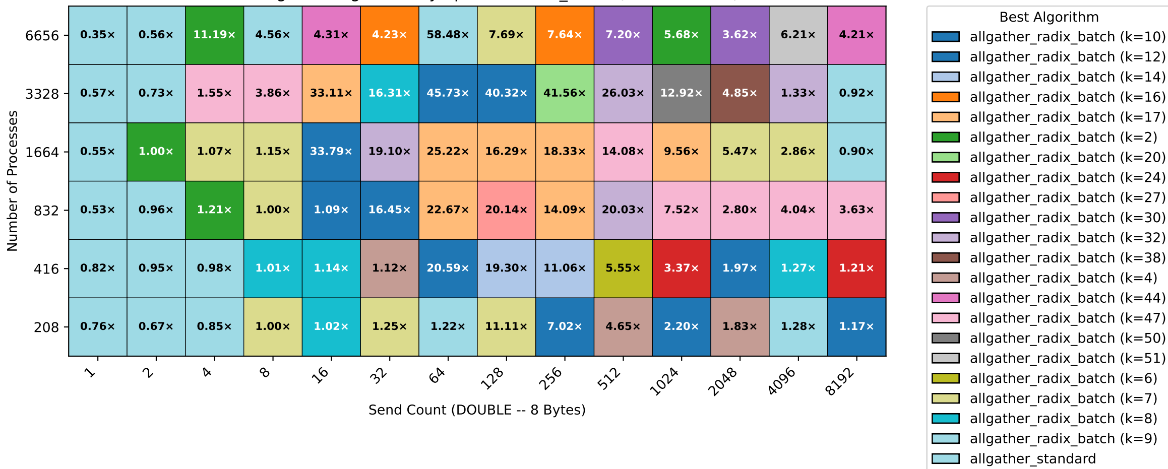
Best Allgather Algorithm by nprocs &amp; send_count (MEDIAN TIME)
