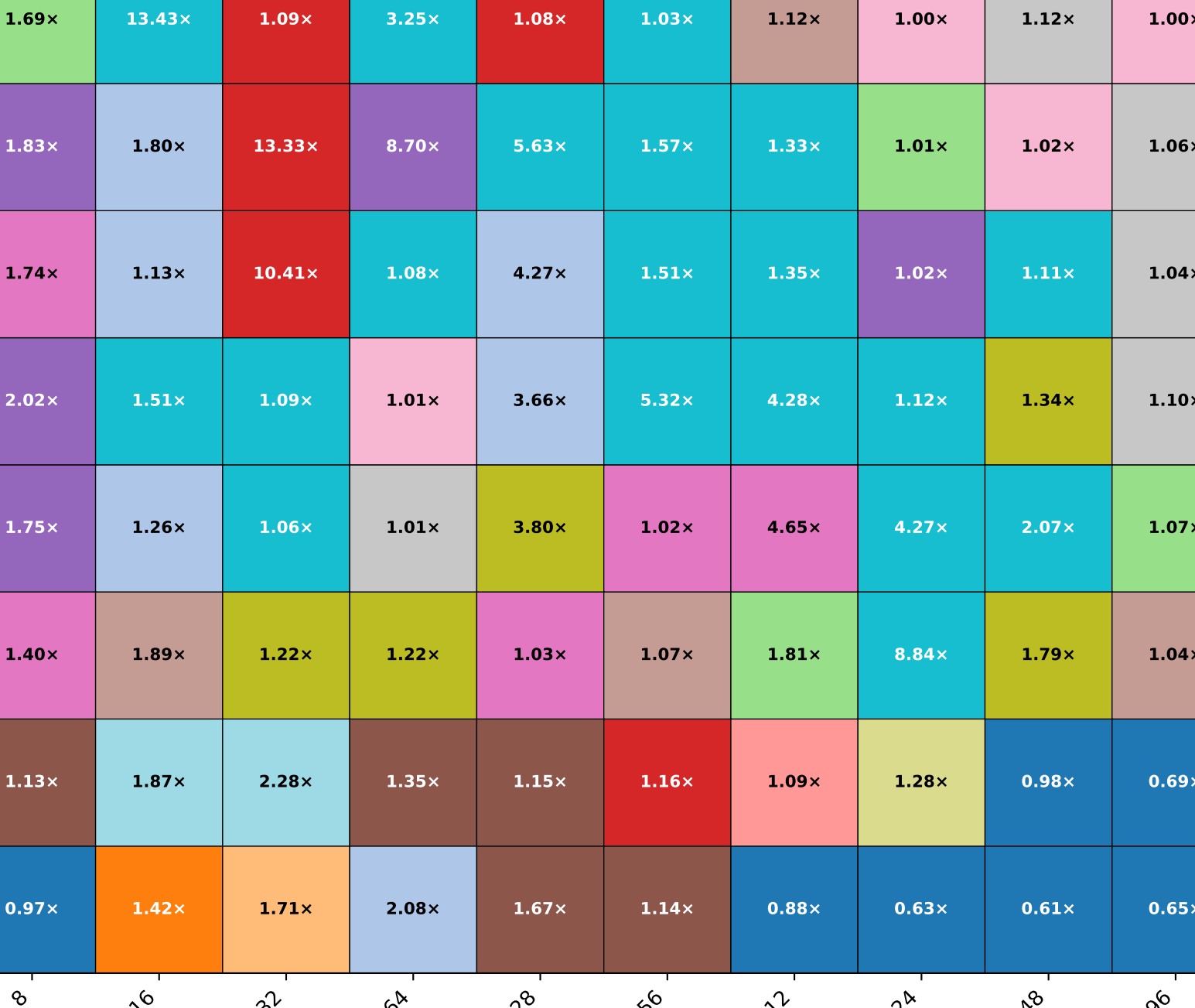
Best Allreduce Algorithm by nprocs &amp; send_count (MEDIAN TIME)
