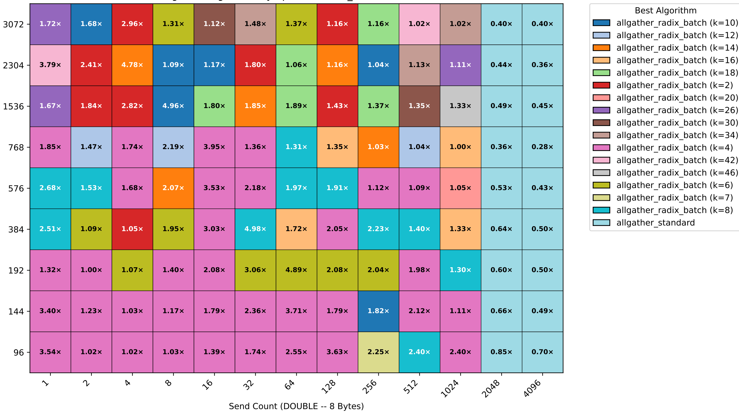
Best Allgather Algorithm by nprocs & send_count (MEDIAN TIME)
