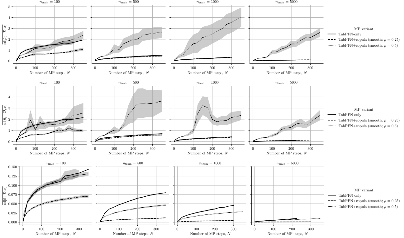
Figure 3. Convergence of different MP variants wrt. increasing number of MP steps N for every nuisance function based on the synthetic data with varying size of the train data, n_{\text{train}} (here d_x = 25 ). Reported: mean posterior standard deviation \text{sd}[\hat{\diamond} | \mathcal{D}, x] \pm \text{se} over 10 runs, where \diamond corresponds to different nuisance functions: (top row) \diamond = \mu_0 , (middle row) \diamond = \mu_1 , and (bottom row) \diamond = \pi^{-1} . Results. We see that, with few exceptions for large \rho , the posterior standard deviation generally flattens with the growing number of MP steps (e.g., for N = 300 with n = 100 , for N = 250 with n = 500 , etc.)
