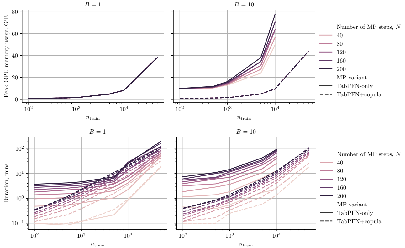
Figure 2. Peak GPU memory usage (top figure, in gigabytes (GiB)) and total runtime (bottom figure, in minutes) of ATE experiments for our MP-OSPC with different MP variants and varying number of MP steps based on the synthetic data with varying size of the train data, n_{\text{train}} (here d_x = 25 ). Experiments are carried out on AMD EPYC 9455 48-Core CPU and 1 H200 Nvidia GPU. Results. While a TabPFN-only MP is very GPU-memory/runtime intensive for increasing number of posterior draws B (as every draw has to be parallelized and requires N subsequent TabPFN calls each with up to O((n + N)^2) time complexity), the copula-based MPs are more GPU-memory/runtime effective (as they require one initial TabPFN call with O(n^2) time complexity and all the MP inference for B draws can be easily vectorized).
