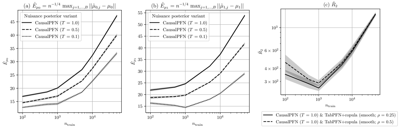
Figure 6. L_2 -convergence check for every nuisance function (a)-(b) and for the second-order remainder \hat{R}_2 (c) based on the synthetic data with varying size of the train data, n_{\text{train}} (here d_x = 25 ). Reported: mean L_2 error \hat{E}_{\diamond}/\hat{R}_2 \pm \text{se} over 10 runs (lower is better), where \diamond corresponds to different nuisance functions: (a) \diamond = \mu_0 , (b) \diamond = \mu_1 (note that propensity score is not available for CausalPFN). Results. These results indicate that performance degrades with increasing sample size for CausalPFN-based functional posteriors \mu_a , as seen in (a)-(b). This is not surprising, considering that CausalPFN was trained on synthetic datasets with up to n \approx 2000 . However, as seen in (c), the second-order remainder \hat{R}_2 converges for n < 1000 . This hints on the double robustness property: the divergence of the CausalPFN-based posteriors for \mu_a can be partially compensated with a convergence of TabPFN-based propensity score MP posterior.
