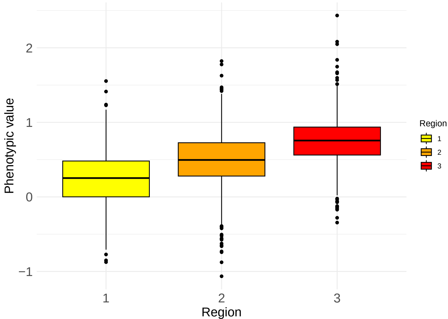
Average phenotypic value by region (Replica 5)
