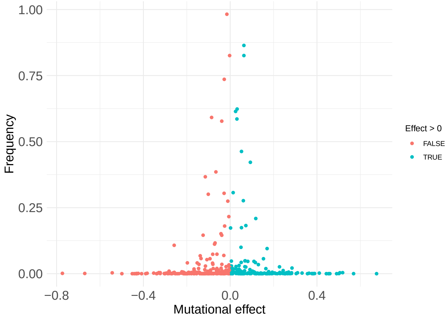
Frequency of Mutational Effects (Replica 5)
