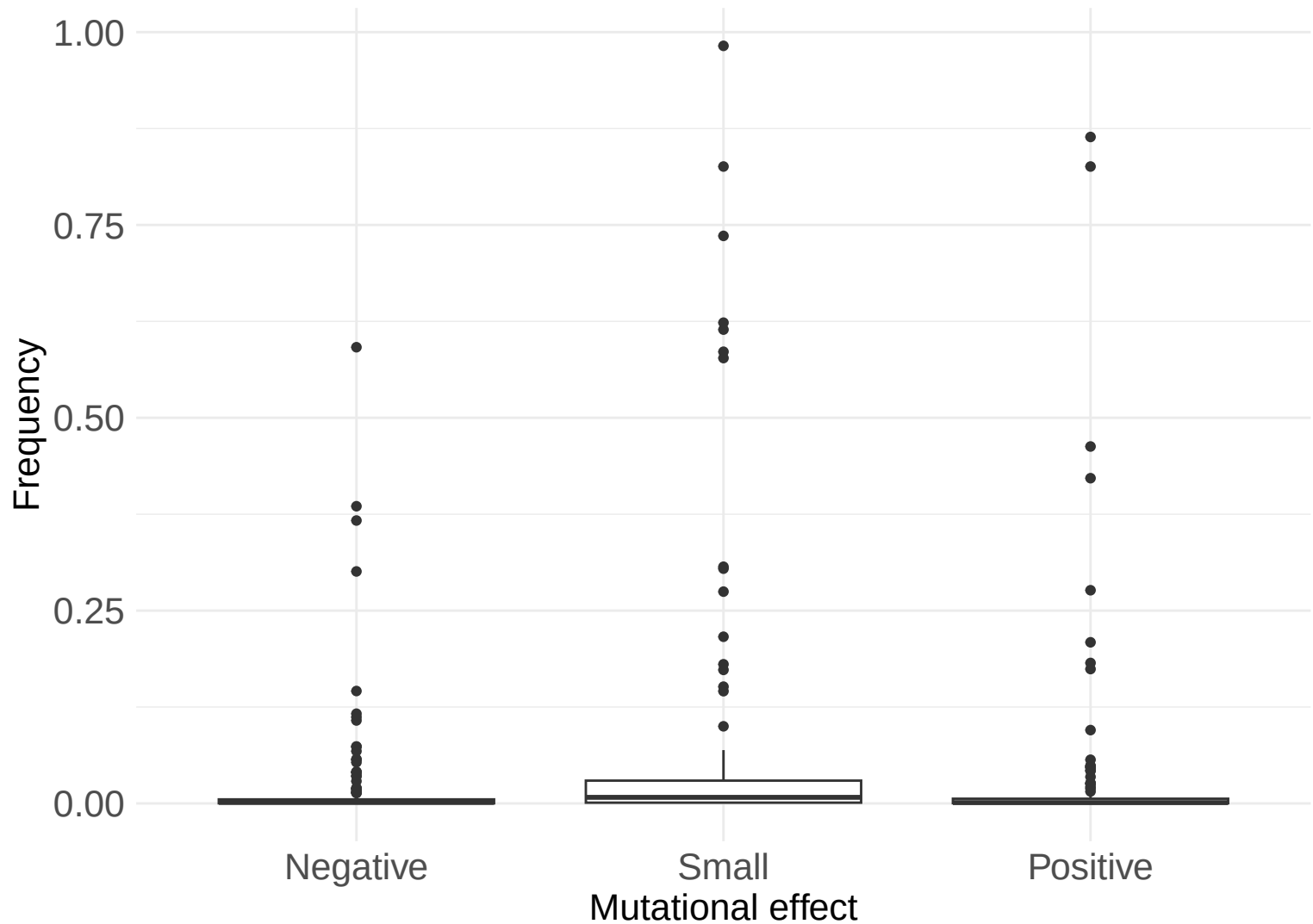
Frequency of Mutational Effects by Group (Replica 5)
