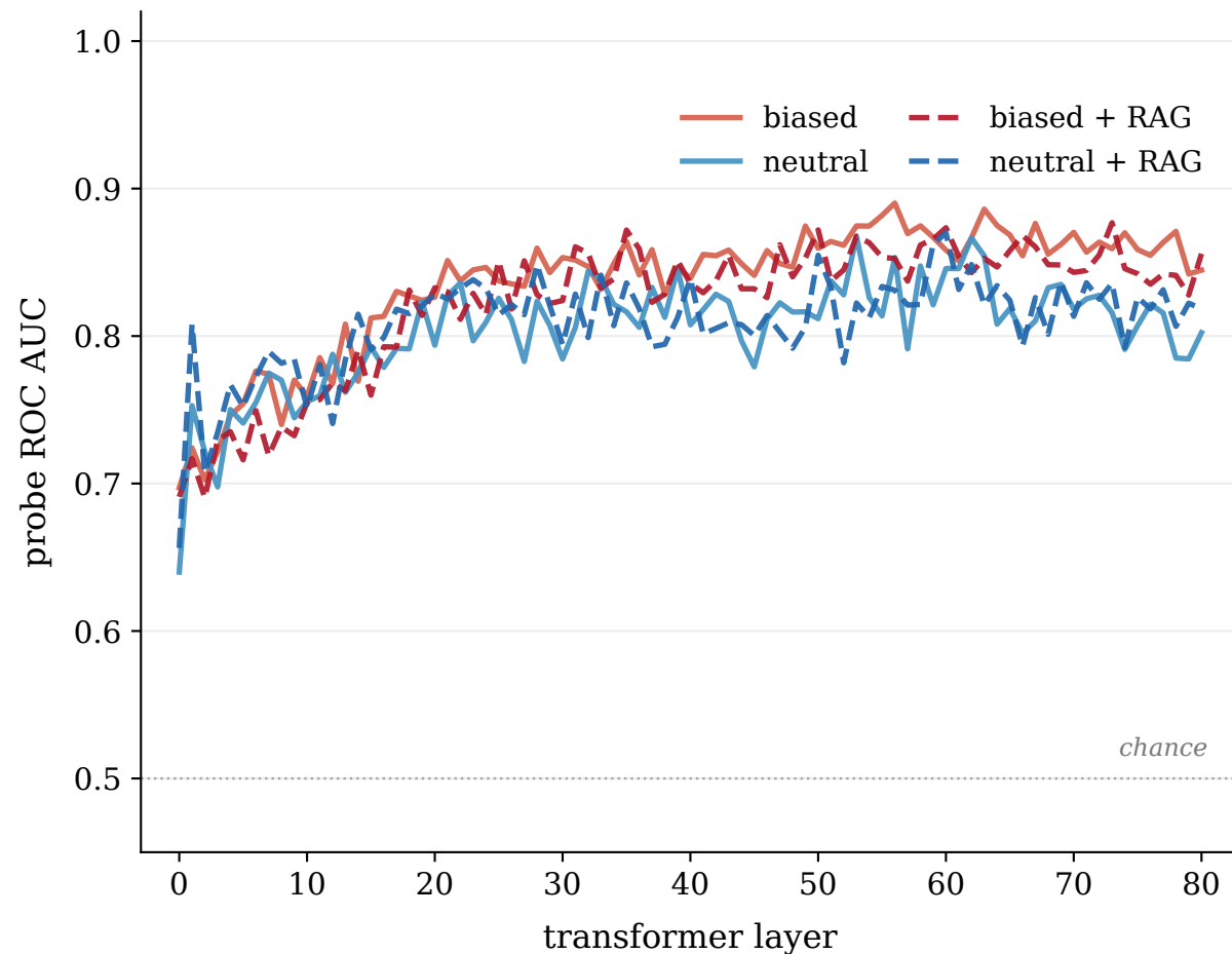
(b) per prompt variant — mean pooling
