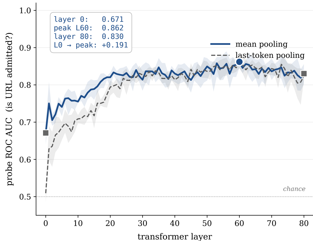
(a) admission probe — pooled over 4 prompt variants
