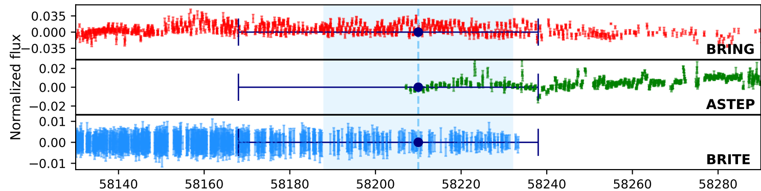
Primary transit at MJD 58210
