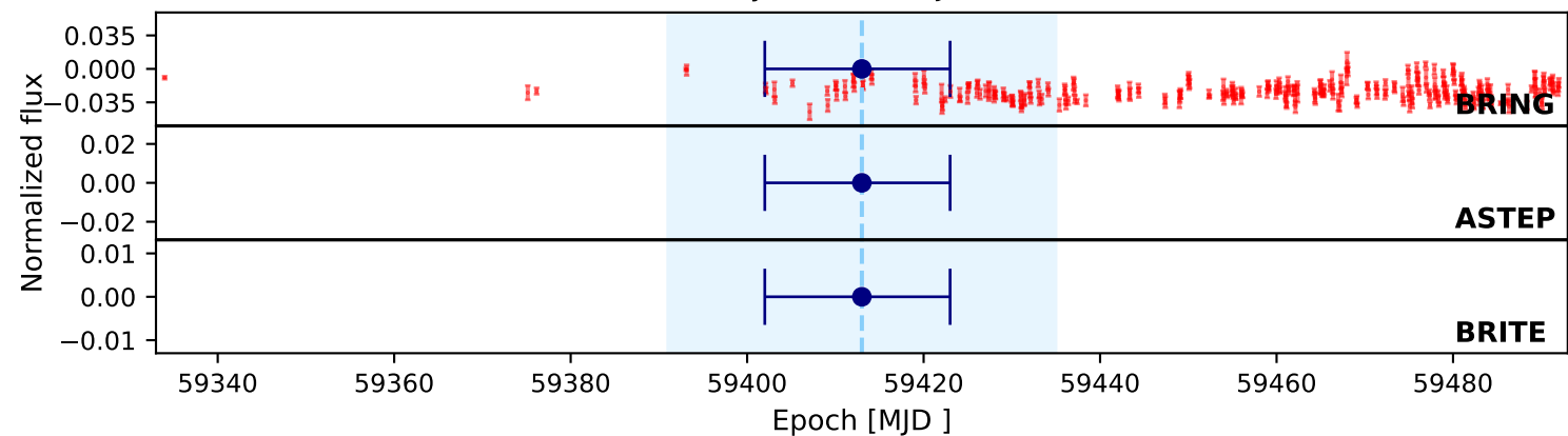
Primary transit at MJD 59413
