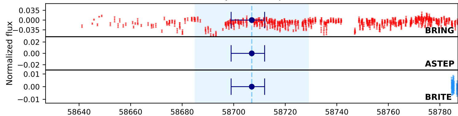
Secondary transit at MJD 58707
