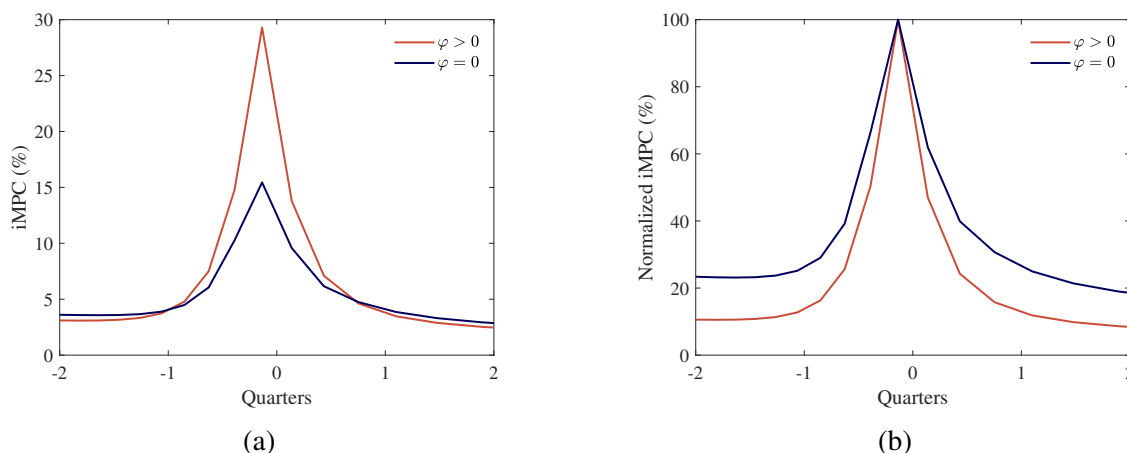
Figure 2: Intertemporal MPCs.
