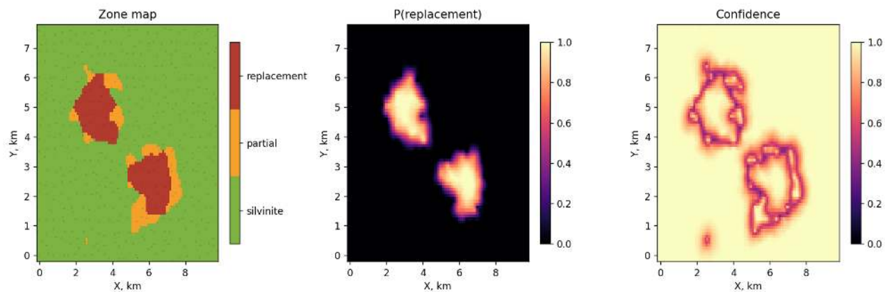
Figure 26: Categorical indicator kriging on a teaching mine: the zone map by maximum probability, the replacement-probability surface and the confidence. Confidence drops along the zone boundaries.
