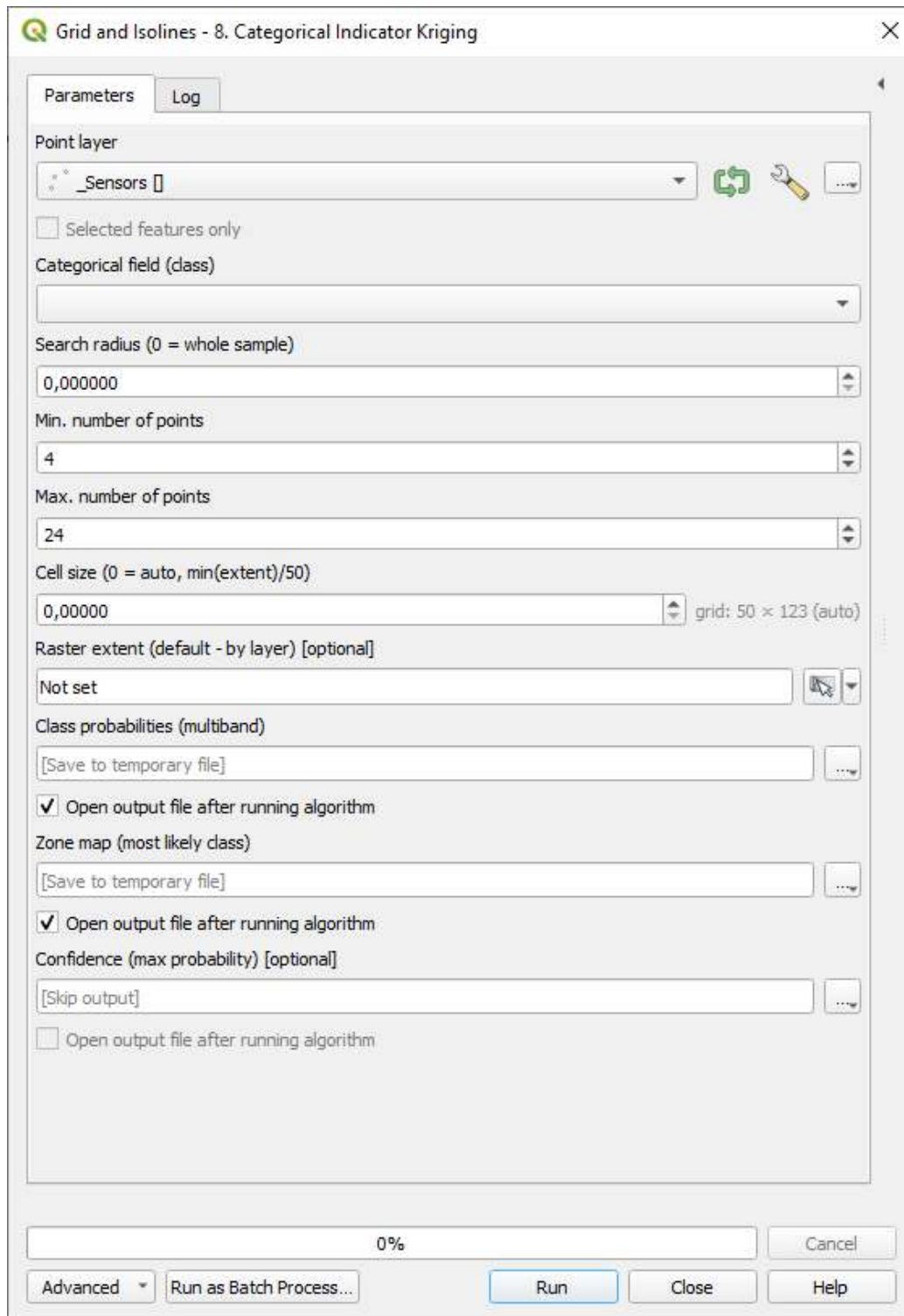
Figure 25: The Categorical indicator kriging dialog.
