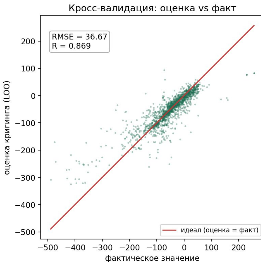
Figure 19: The idea of cross-validation: the kriging estimate from the remaining points (vertical) is compared with the actual value (horizontal). The tighter the cloud lies on the estimate = actual diagonal, the more accurate the prediction.
