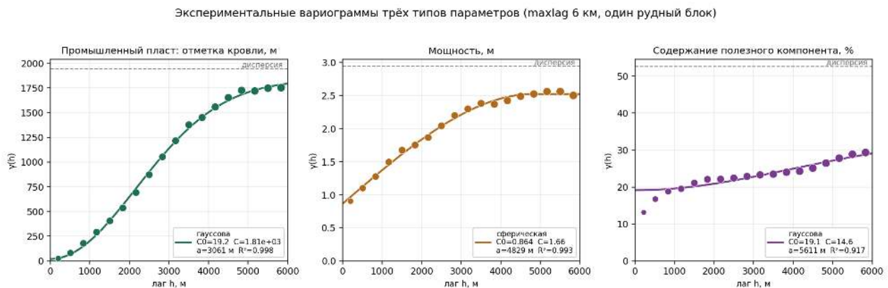
Figure 16: Three parameter types of one seam in a single window: roof elevation (almost zero nugget, smooth surface), thickness (nugget about a third, spherical) and grade (nugget comparable to the contribution, a noisy parameter).
