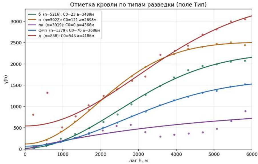
Figure 15: Roof elevation for the KrII seam, grouped by survey type: the underground network lies noticeably lower (a more homogeneous area), the detailed survey gives a high nugget. The different populations are visible at once.
