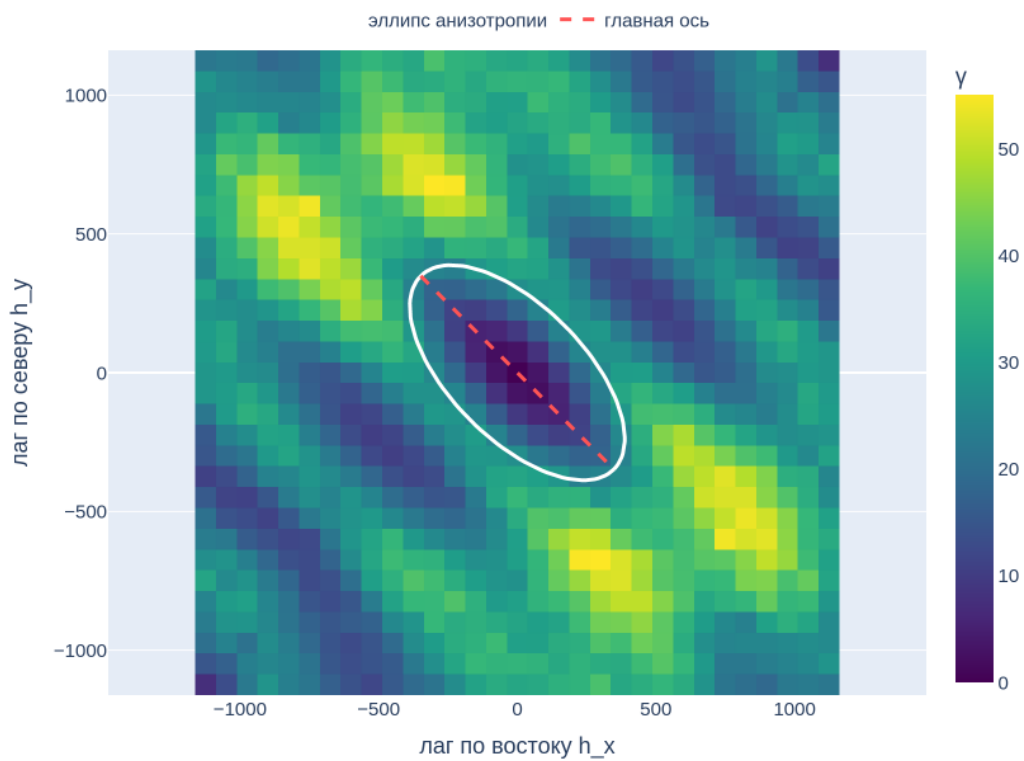
Figure 17: A variogram map: the dark (low \gamma , high continuity) area is elongated at an azimuth of about 135^\circ . The white ellipse and the red dashed major axis show the estimated direction and anisotropy.
