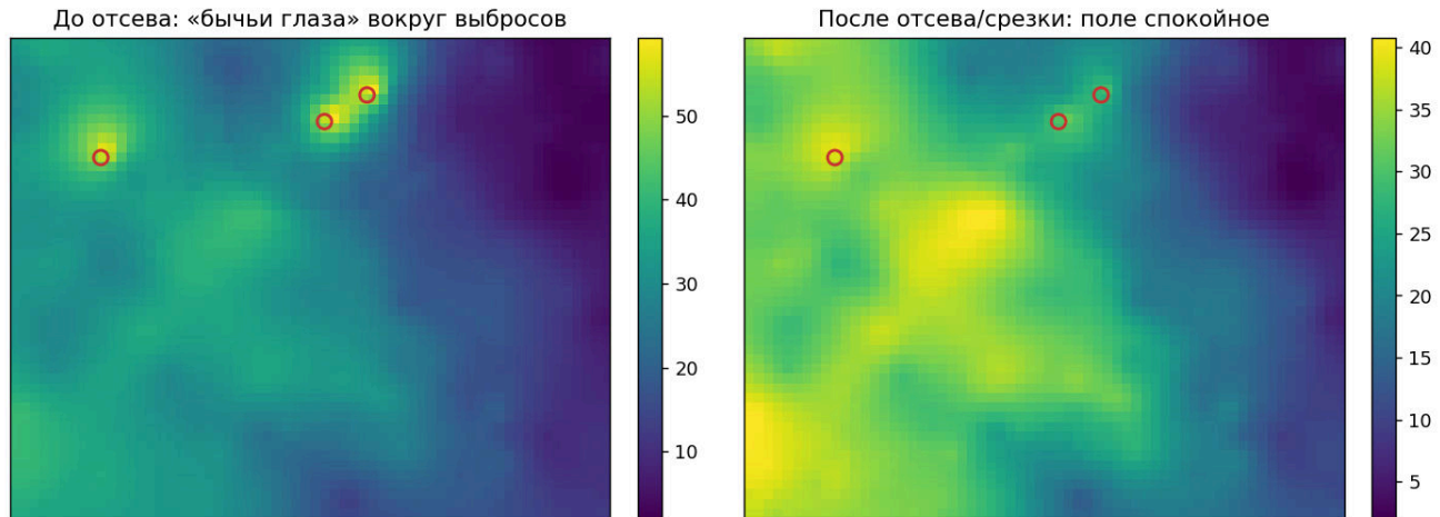
Figure 9: Outlier removal by example: on the left three outliers give “bull’s eyes” (hot spots), on the right after capping to the upper bound the field is calm.
