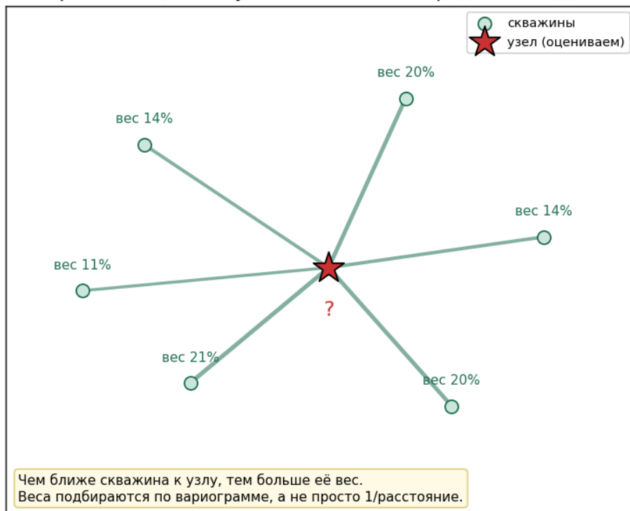
Figure 3: Kriging estimates the node value as a weighted mean of the nearest wells: the closer the well, the larger its weight. Weights come from the variogram.
