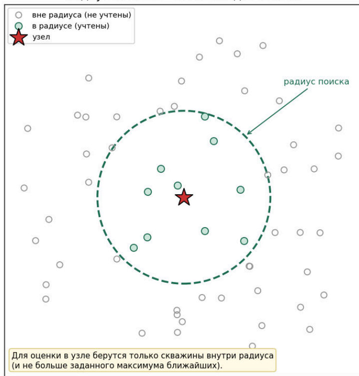
Figure 4: For each node only wells within the search radius are taken, and no more than the set number of nearest ones. Points beyond the radius do not take part.
