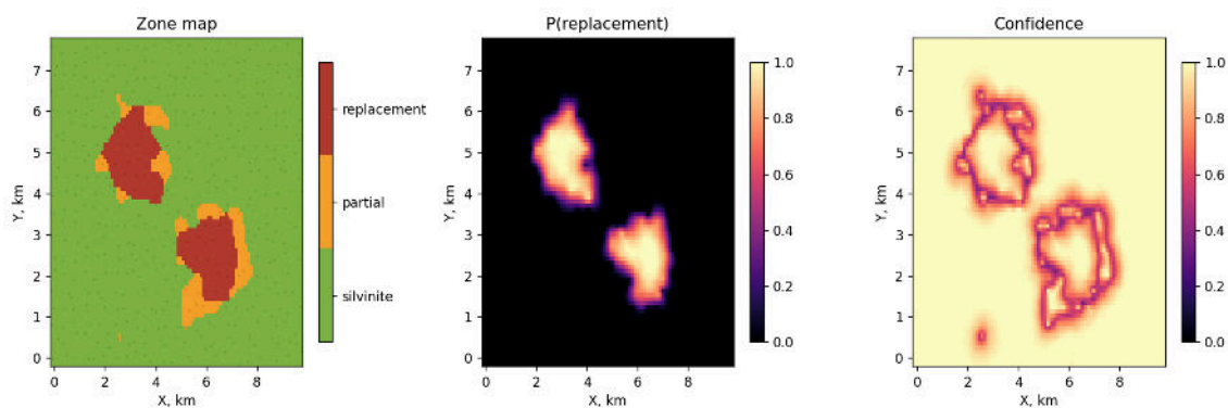
Figure 23: Categorical indicator kriging result: a map of the most likely mineral type, a silvinit background with replacement spots, boreholes drawn on top.
