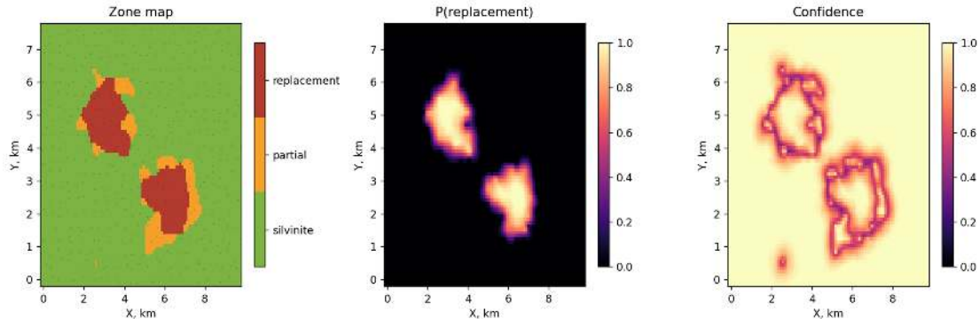
Figure 32: Categorical indicator kriging result: a map of the most likely mineral type, a silvinitite background with replacement spots, boreholes drawn on top.
