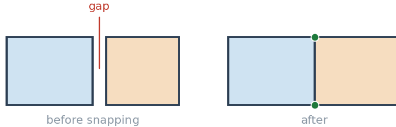
Figure 4: A gap below the tolerance is closed by merging vertices.
