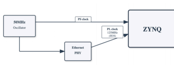
FIG 3.3 - ZYNQ Clock Distribution Architecture
