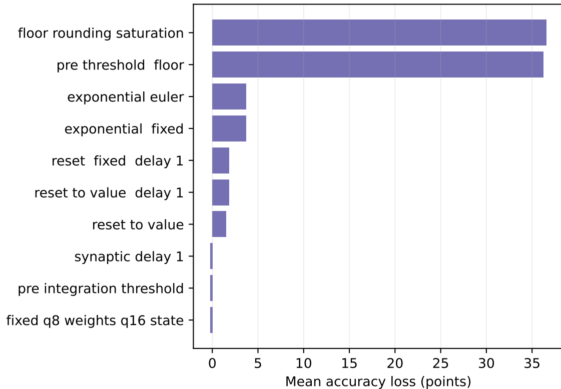
Floor-rounded fixed point dominates loss
