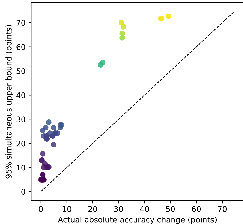
Coverage holds, but bounds remain loose
