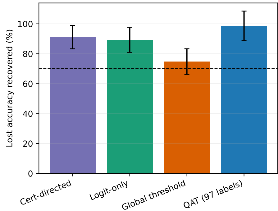
DVS fixed-point repair
