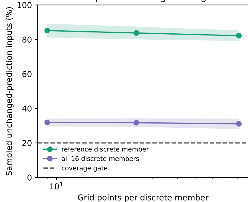
Empirical coverage ceiling
