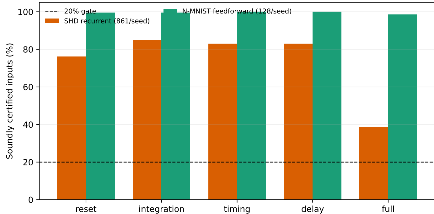
Static-family certificate contrast across trained models
