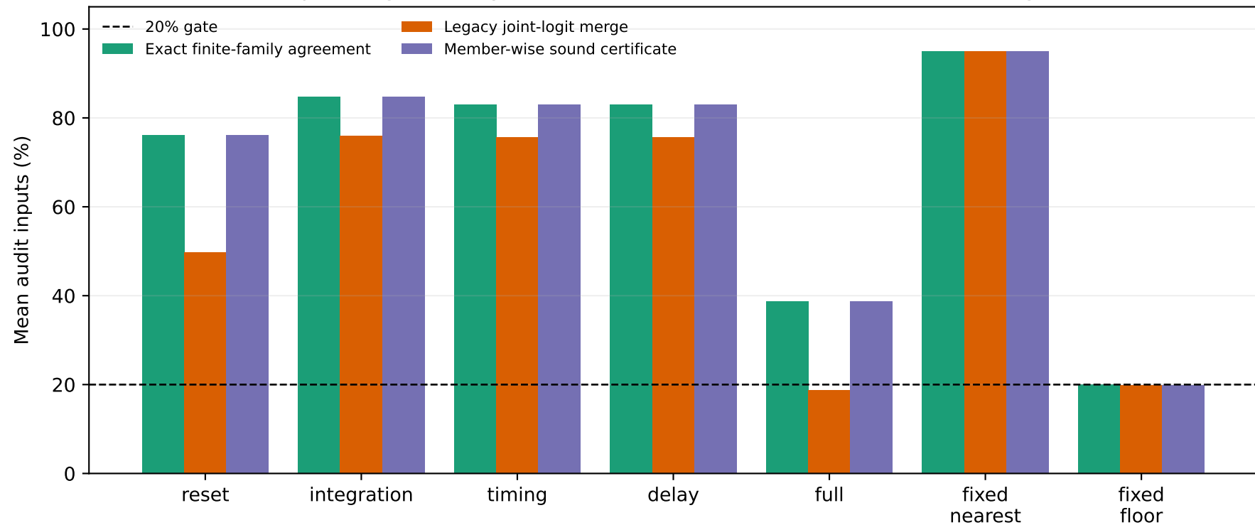
Separating mutually exclusive semantics reverses the SHD static gate
