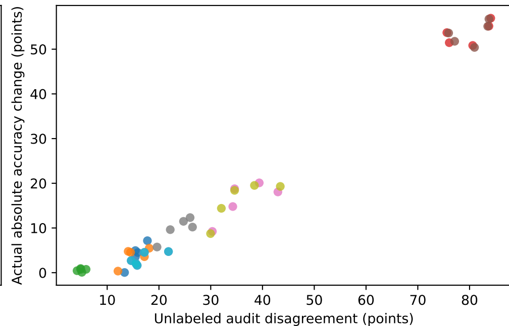
Predictive ranking, not a tight bound ( r=0.989 )
