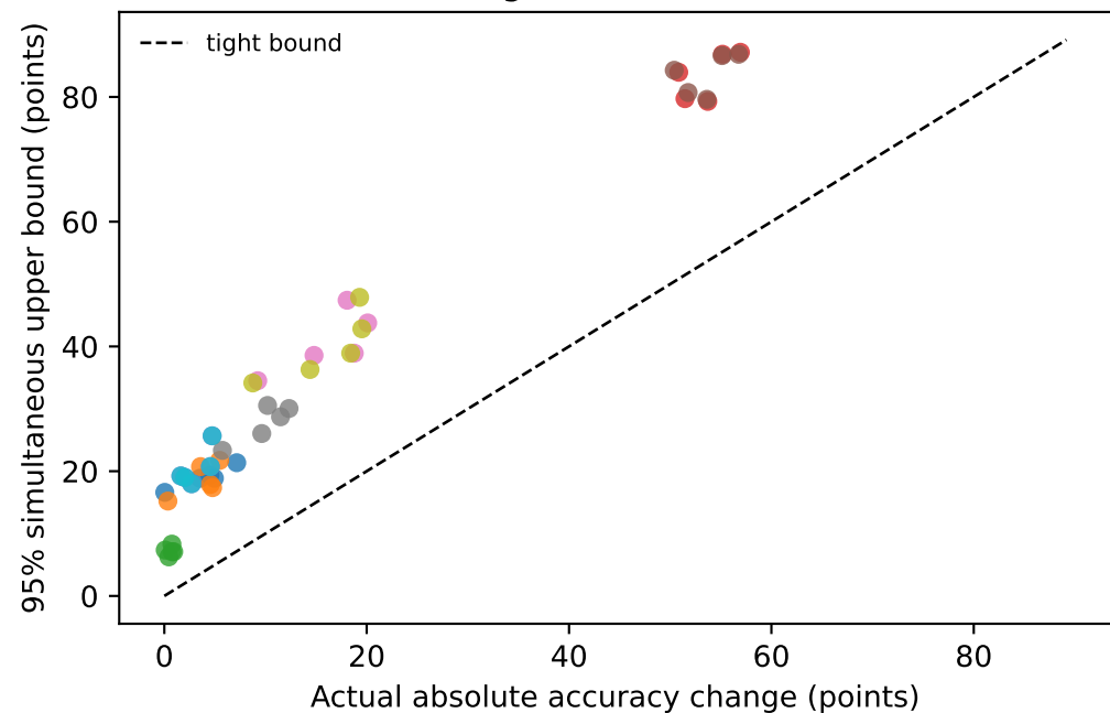
Coverage is valid but loose
