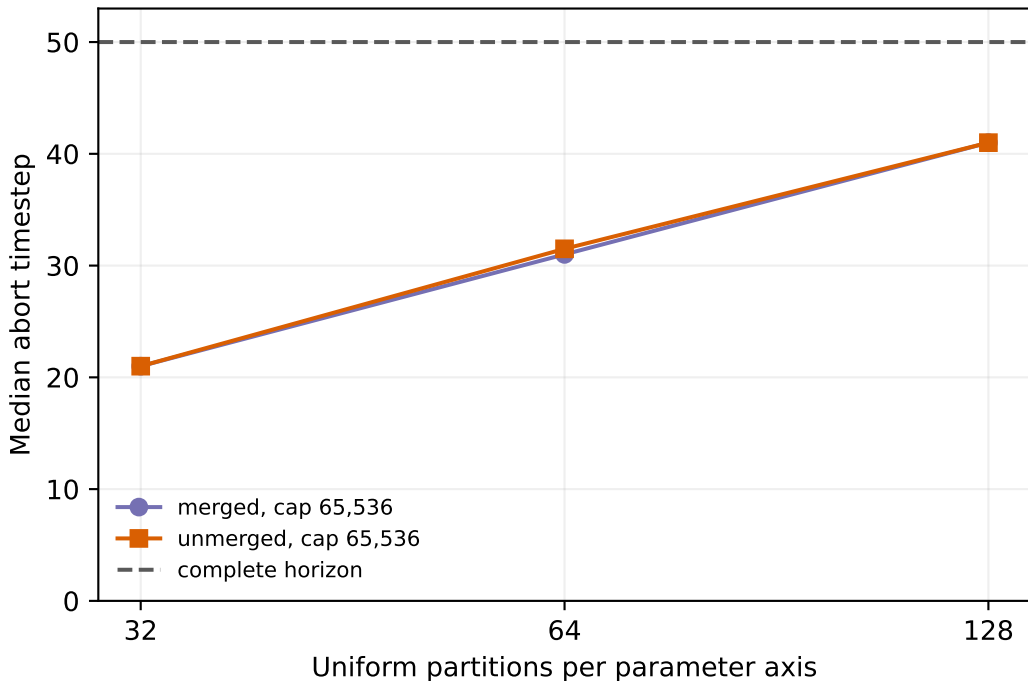
Explicit branch sets remain incomplete
