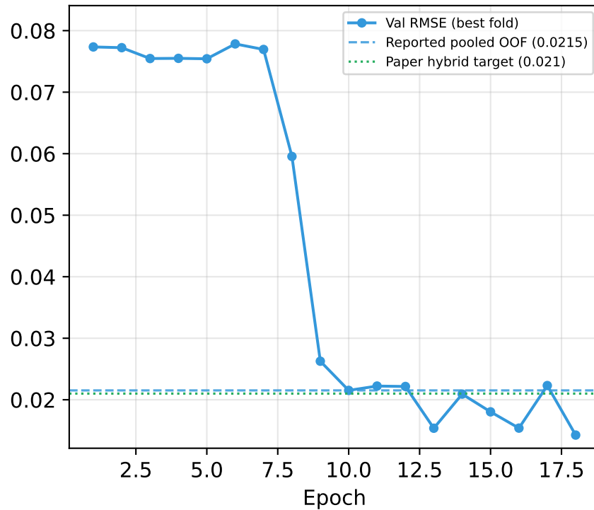
Training Convergence (best CV fold, up to early-stopping epoch)
